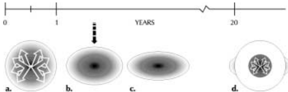
Figure 3. Gentry's Model of dual elliptical/circular halo formation in coalified wood (see text for description)
